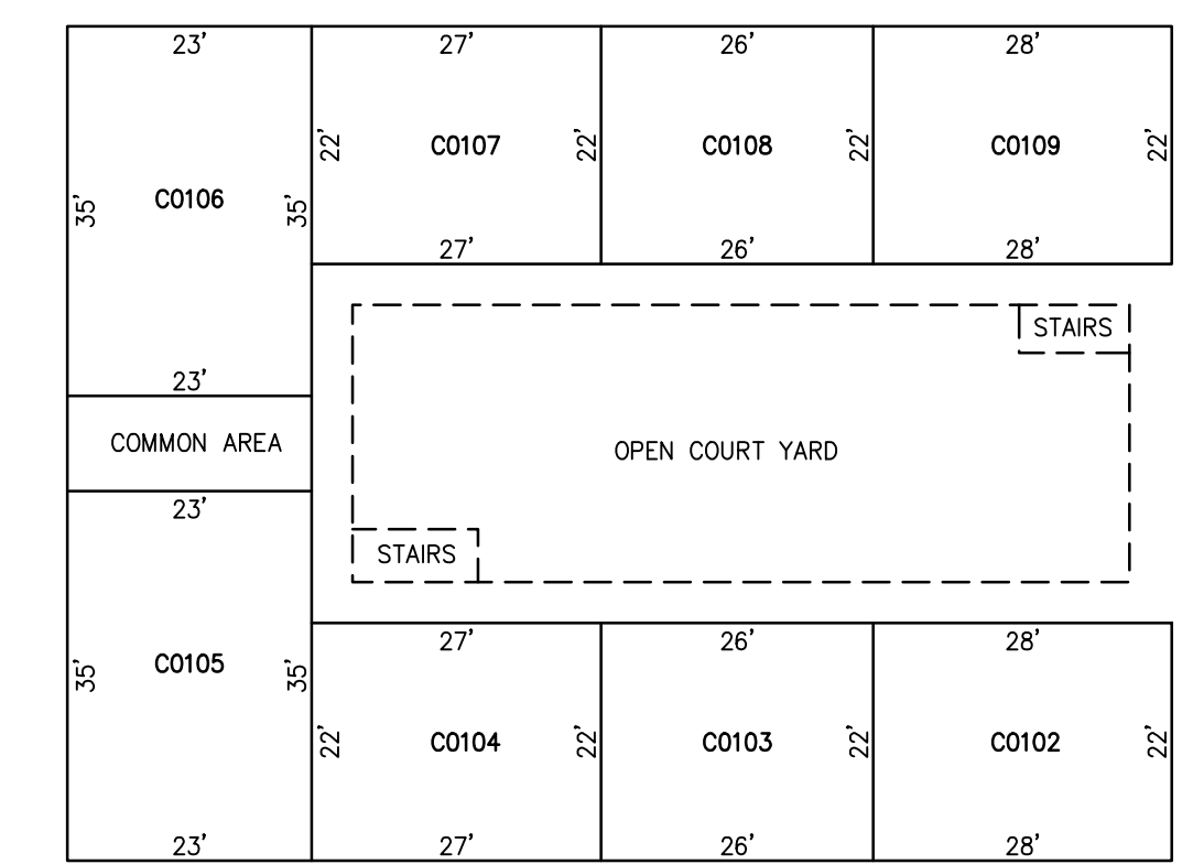
SECOND FLOOR
