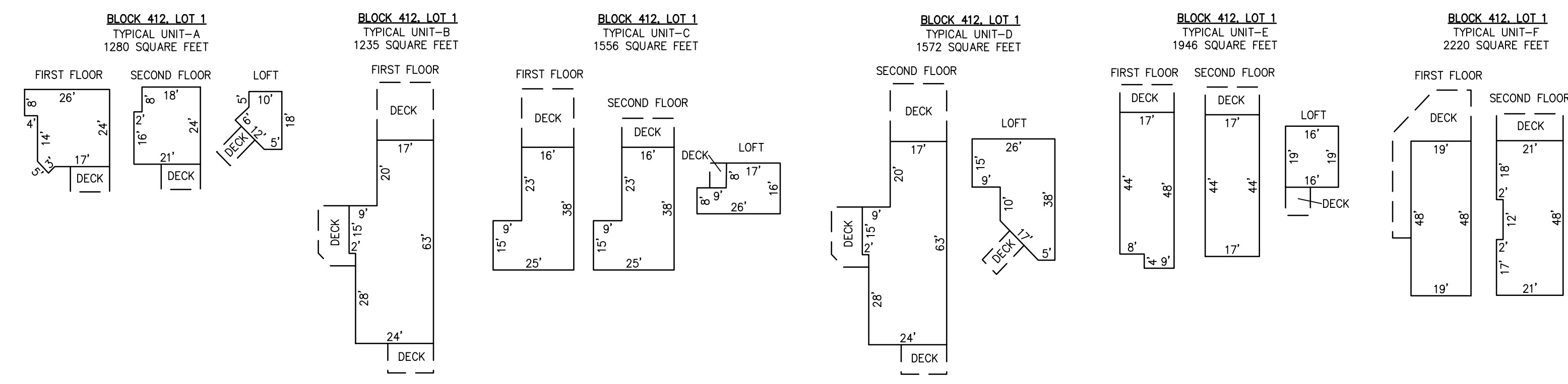
DETAILS SCALE: 1"=30' BLOCK 412, LOT 1 CROWN KEY YACHT CLUB CONDOMINIUM
